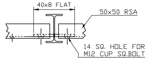
SECTION THRU POST
