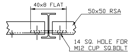
SECTION THRU POST
